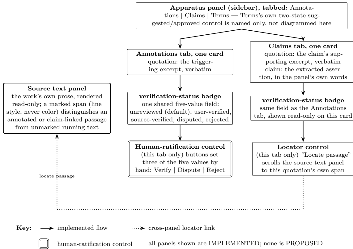
Fig. 4. The reference implementation's verification-relevant panels, as implemented, derived by direct inspection of its own front-end component code rather than drawn from a screenshot – no color, layout proportion, or literal screen composition is reproduced, only panel structure, control affordances, and status vocabulary. The source text panel at left renders the work's own prose read-only; an in-line marker, never color alone, distinguishes an annotated or claim-linked span. The apparatus panel (sidebar) carries additional non-verification tabs not shown here – Critical notes, a separately-named Apparatus tab, Sources, and My notes. Of its verification-relevant tabs, two are shown side by side, disclosed here as two separate cards rather than one combined view, since that is how the live interface actually separates them. The Annotations tab's card carries a verbatim triggering excerpt and, below it, this architecture's five-value verification-status field — unreviewed by default, then user-verified, source-verified, disputed, or rejected — of which only three (Verify, Dispute, Reject) are settable by a button on this same card, a distinction the figure states explicitly rather than implying all five are equally reachable by hand. The Claims tab's card instead pairs a verbatim supporting excerpt with the extracted claim text and the same shared status field shown read-only, plus a locator control ("Locate passage") that scrolls the source text panel to that quotation's own span, drawn as a dotted cross-panel link back to the leftmost panel. A third tab, Terms, exists in the same apparatus panel with its own, differently-scoped two-state suggested/approved control and is named but not separately diagrammed. Every element shown is IMPLEMENTED in the reference implementation as inspected; this figure depicts no PROPOSED construct.
